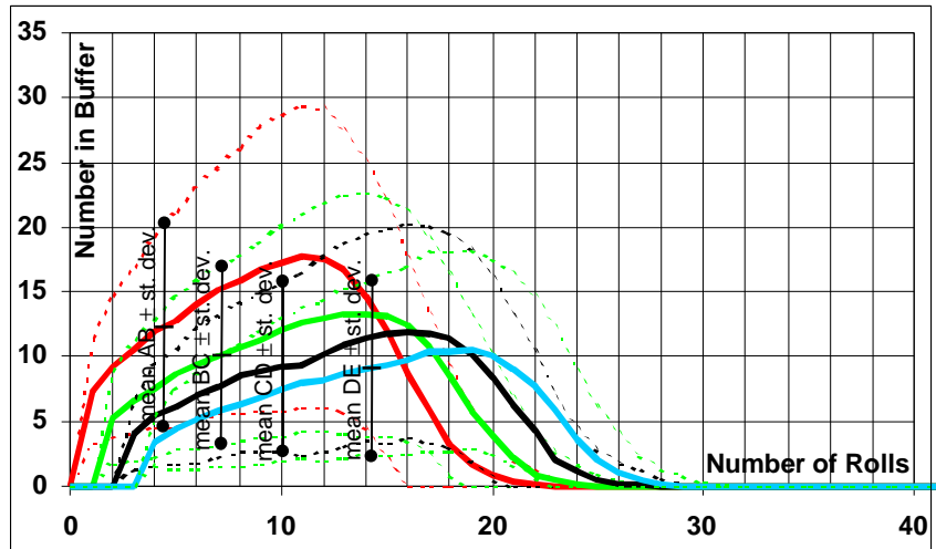
Figure 11: Average \pm Standard Deviation of Buffer Size Relative to Number of Rolls after 1,000-Iteration Simulation where all Players have a fast Die (3-11)
